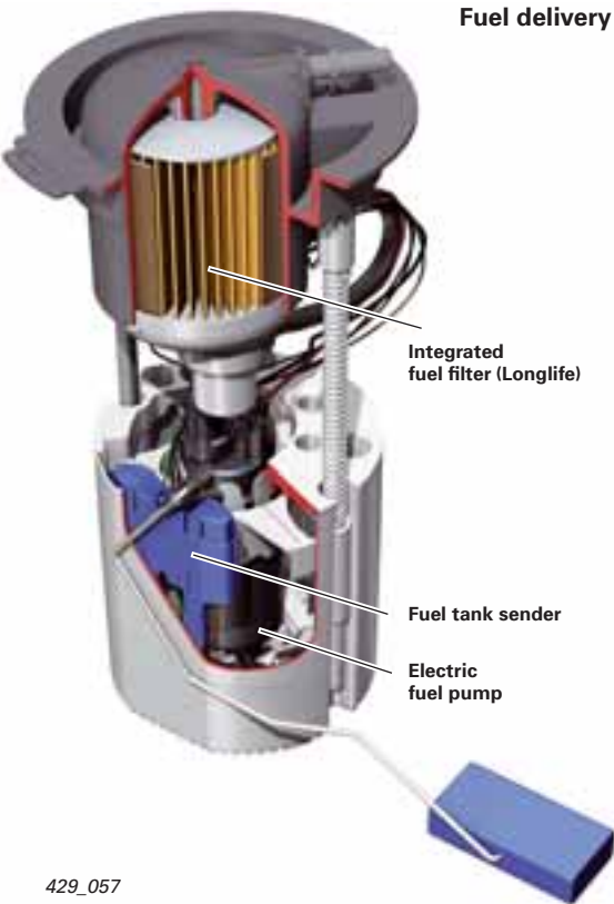
Fuel delivery unit for FSI engine
