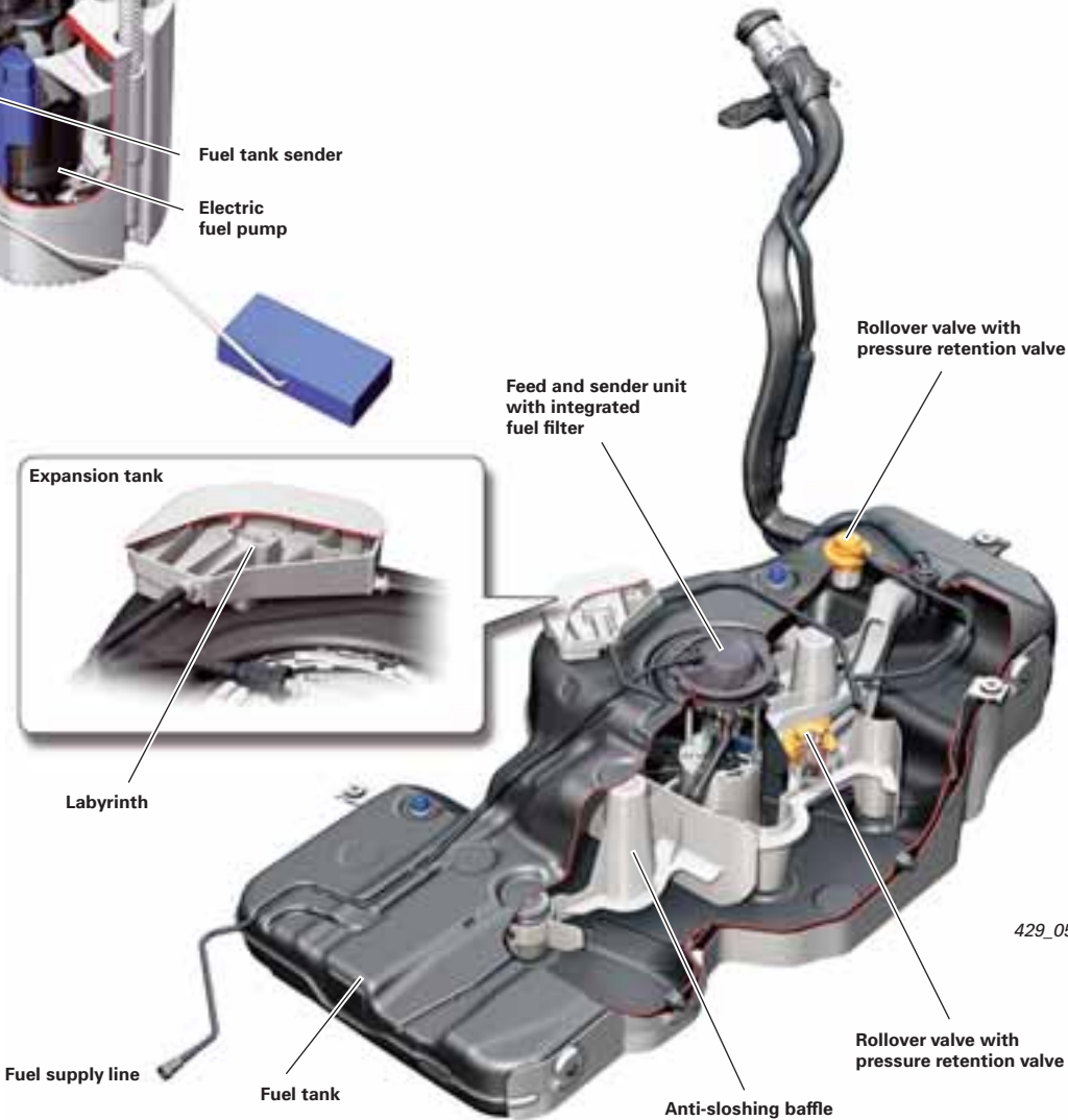
FSI fuel tank
